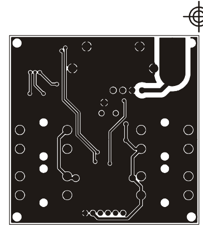
CDP-TX-04S-TestBoard 16670
