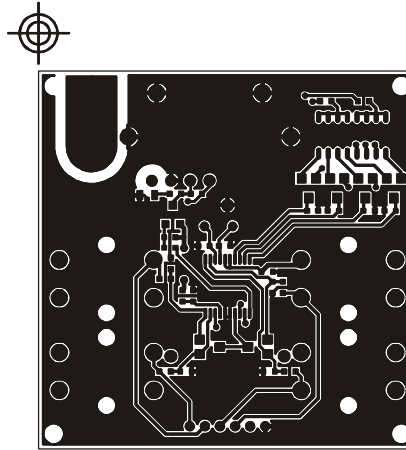
CDP-TX-04S-TestBoard 16670
