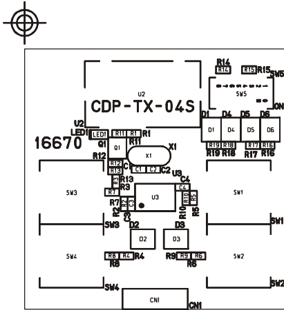
CDP-TX-04S-TestBoard 16670
