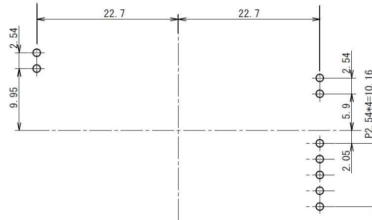
Reference hole position for PCB mounting (Top view)
